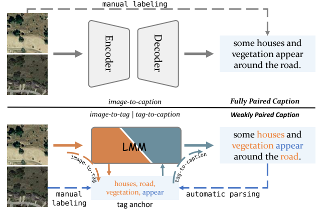
Fig. 1: Comparison of the conventional fully-paired paradigm (top) with our factorized, weakly-paired approach (bottom). The former requires costly end-to-end image-to-caption alignment, while WeCap introduces intermediate tag anchors — what changed and how it changed —to decouple the task into data-efficient image-to-tag perception and tag-to-caption interpretation stages.
