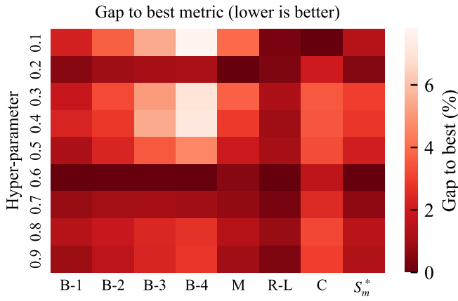
Fig. 3: Sensitivity analysis of the synonym replacement probability, p_{replace} , used in our Linguistic Alignment task. The heatmap visualizes the percentage gap to the best-achieved score for each metric across different probability values. Darker red indicates a smaller gap and thus better performance.
