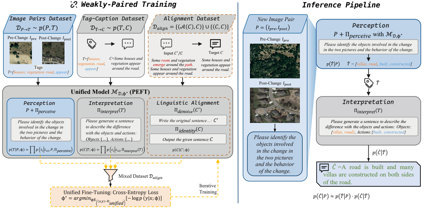
Fig. 2: Overview of our WeCap framework’s training and inference process. Our approach leverages a single Large Multimodal Model, fine-tuned on a mixture of three weakly-paired data sources to learn three distinct capabilities: Perception (image pair \rightarrow tags), Interpretation (tags \rightarrow caption), and Linguistic Alignment (paraphrase \rightarrow canonical caption). Each capability is invoked by a specific prompt. During inference, the trained model operates in a seamless two-stage pipeline: it first perceives a set of semantic tags from a new image pair, and then interprets these tags to generate the final, descriptive caption.
